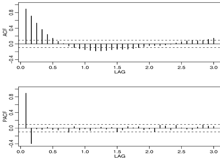
Fig. 5.12. ACF and PACF of the estimated noise \hat{\eta}_t departures from the transfer function model.
